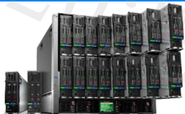
Cloud Servers
